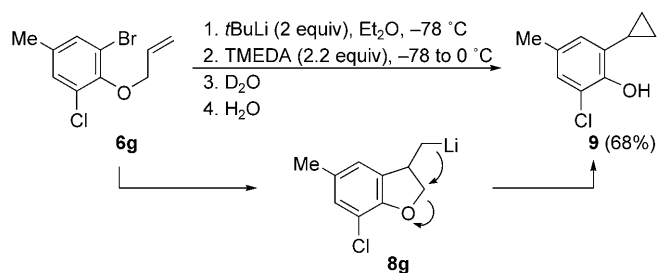
Scheme 4. Formation of o -cyclopropylphenol derivative 9 from 6-chloro-substituted aryl ether 6g .
