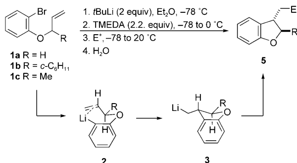
Scheme 2. trans -2,3-Dihydrobenzofuran derivatives 5 from allyl 2-bromophenyl ethers 1 through intramolecular carbolithiation of organolithium compounds 2 .
