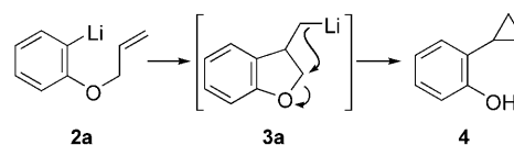
Scheme 1. Tandem carbolithiation/1,3-elimination reactions of allyl 2-lithiophenyl ether 2a .
