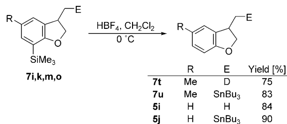
Scheme 5. Protodesilylation of 7-trimethylsilyl-substituted 2,3-dihydrobenzofurans 7i,k,m,o .
