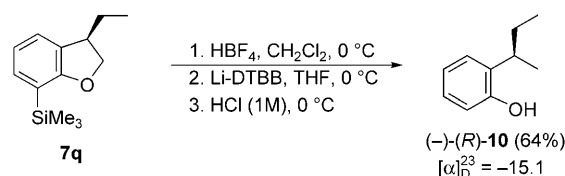
Scheme 6. Chemical correlation of 3-ethyl-7-trimethylsilyl-2,3-dihydrobenzofuran 7q with (–)-( R )-2- sec -butylphenol.
