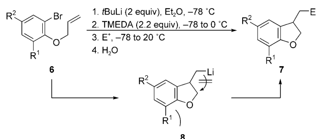
Scheme 3. Formation of dihydrobenzofuran derivatives 7 from 6-substituted aryl ethers 6 .
